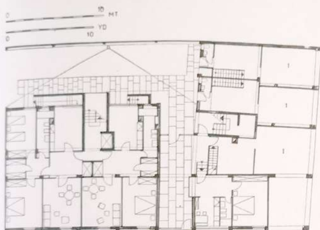
Pianta del piano terreno Ground floor plan
