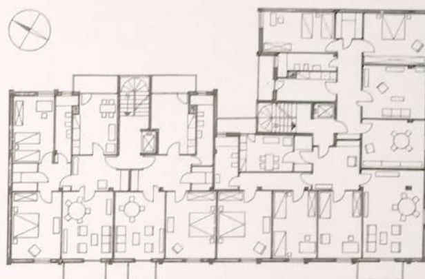
Pianta del piano tipo Typical floor plan
